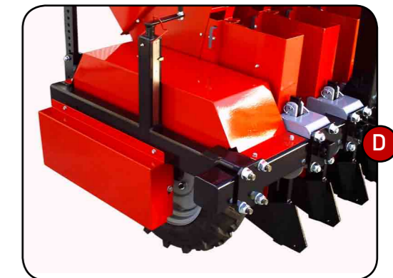
D. Driven wheels adjusted to different seed beds height (option).
